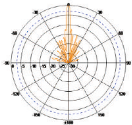
H-Pol Elevation
