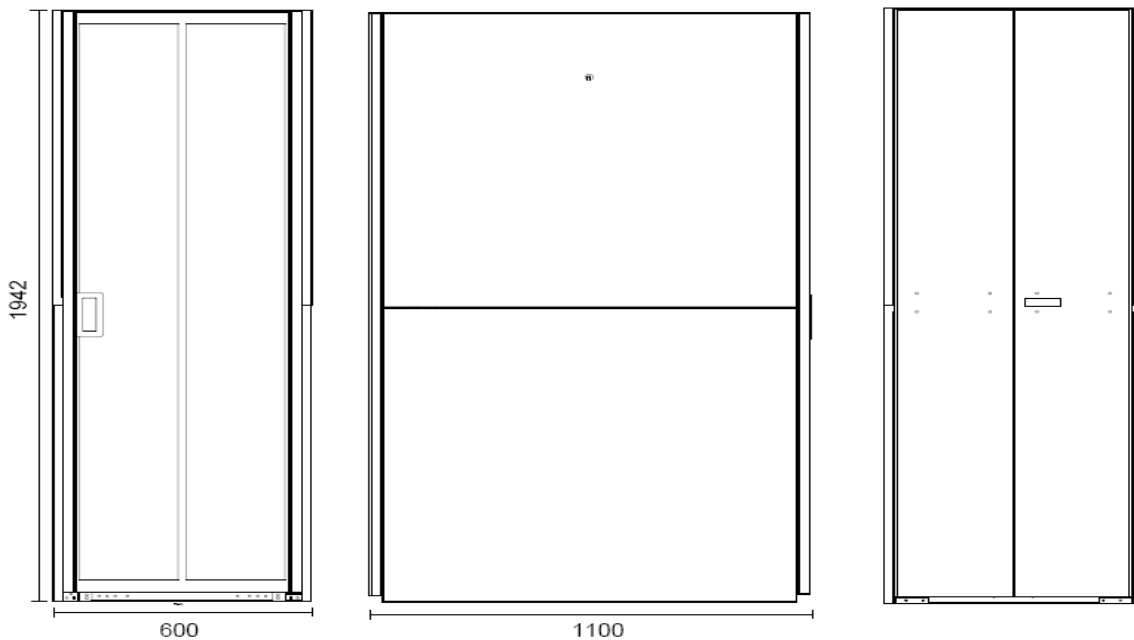
Top view
