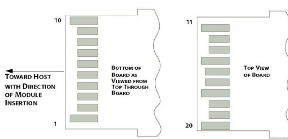
Figure 3: Module Contact Assignment
