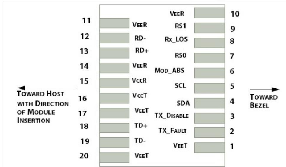
Figure 2: Interface to Host PCB
